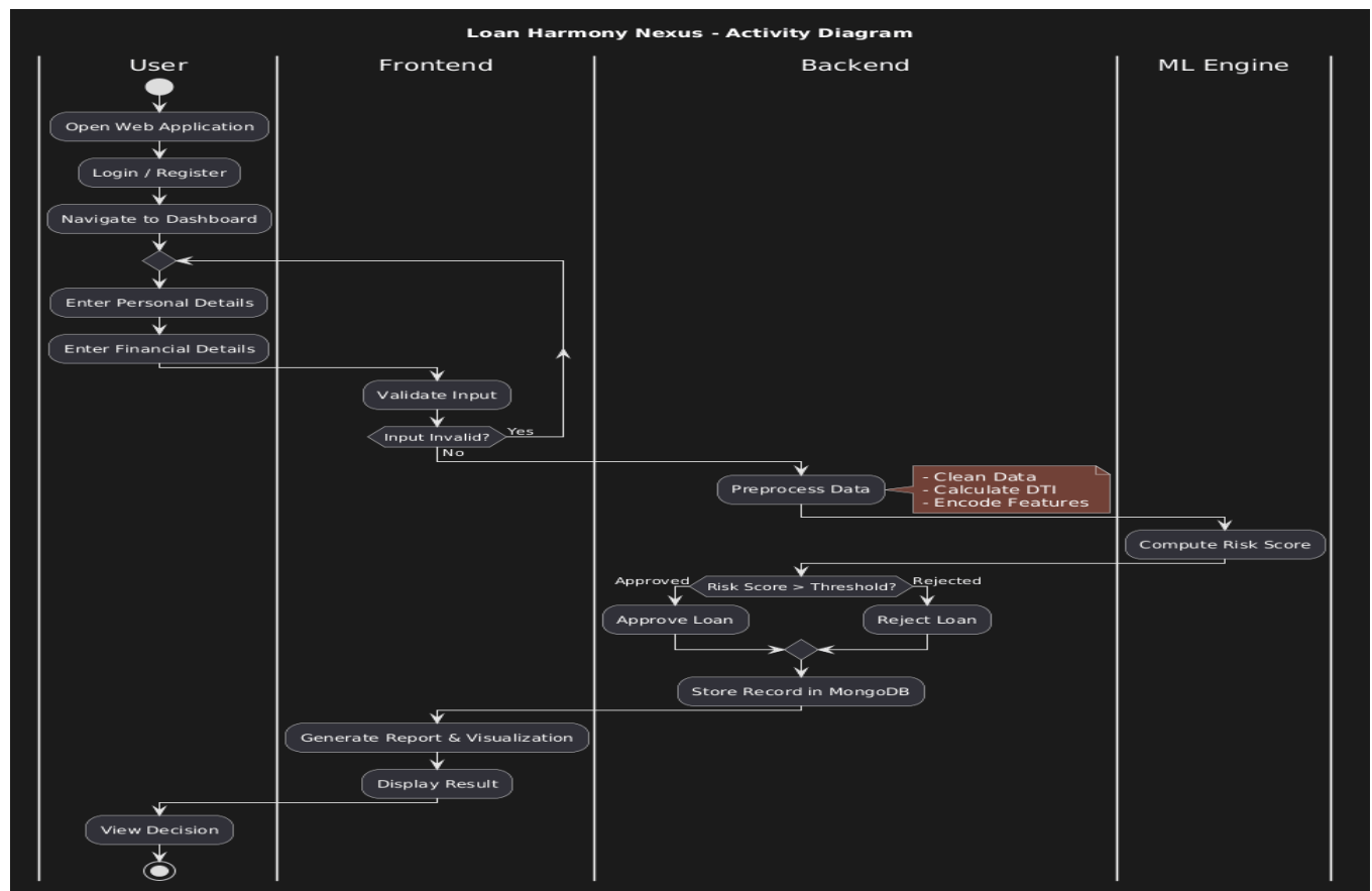
Fig 3.2: Activity Diagram
