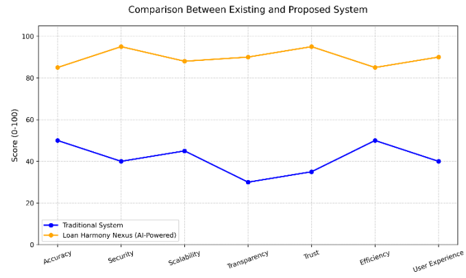
Fig 3.4: Comparison Graph
